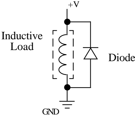
Typical circuit showing a flyback diode installed across an inductive load. (Relay Coil, Solenoid, etc.)
