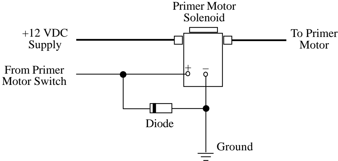
Diagram showing a flyback diode connected on a typical pump primer motor solenoid.
